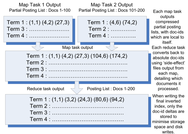
Figure 1: Correcting document IDs while merging.
